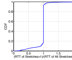
Figure 6: Delayed ACK effect on Data-ACK RTT
