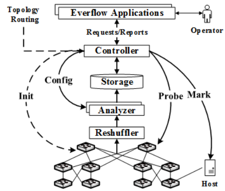
Figure 4: Everflow architecture
