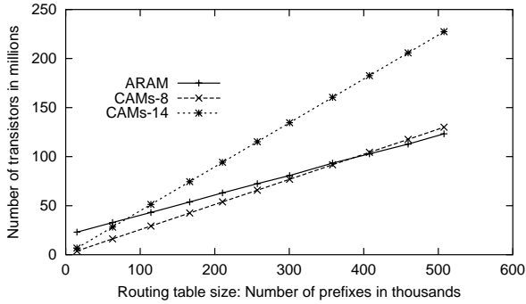
Figure 8: The size of the routing table is increased by increasing the number of allocations (other parameters are kept constant). We see that unless TCAMs use 8 transistors per cell or less, multibit tries would use lesser transistors than TCAMs.
