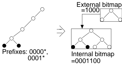
Figure 5: This figure shows an example of a unibit trie on the left and its corresponding multibit version on the right; for the prefixes 0000* and 0001*. The bitmaps of the Tree Bitmap Algorithm for the multibit version are also shown. The memory required is 45 bits.
