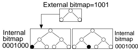
Figure 6: This figure shows what happens if the prefixes change to 0000* and 1101*. Now, two child nodes are required. The external bitmap is 1001 because the the first and the last child nodes of the root exist. The memory required is 73 bits.
