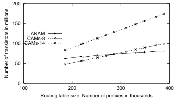
Figure 11: The size of the routing table is increased by increasing F_{split} (other parameters are kept constant). We see that multibit tries scale better in this case. This is because load shared prefixes are clustered together - more than multihoming assignments.
