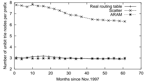
Figure 4: Unibit Trie Density
