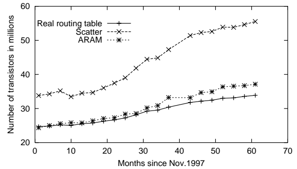
Figure 7: The memory used by the multibit trie by the real routing table, scatter and ARAM.
